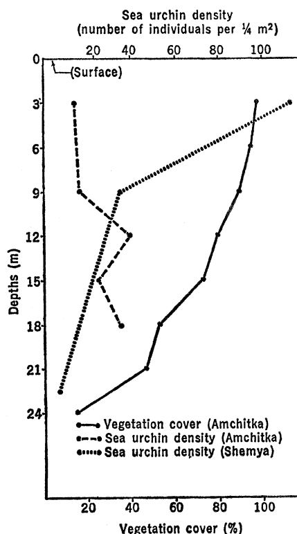
Fig. 1. Vegetation coverage and sea urchin density plotted against depth. The data for Amchitka Island and Shemya Island represent averages from four and three study areas, respectively. Vegetation cover at Shemya Island is coincident with the ordinate.
